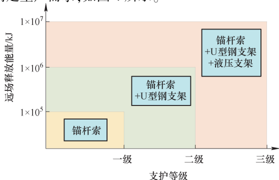
图4 防冲支护体系 Fig.4 Anti-rockburst prevention support system
